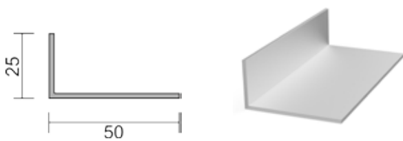
SP L2550 L-profile 25 x 50 x 2 mm
