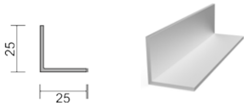
SP L2525 L-profile 25 x 25 x 2 mm
