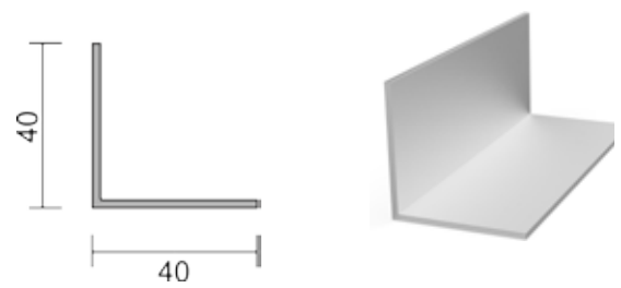
SP L4040 L-profile 40 x 40 x 2 mm
