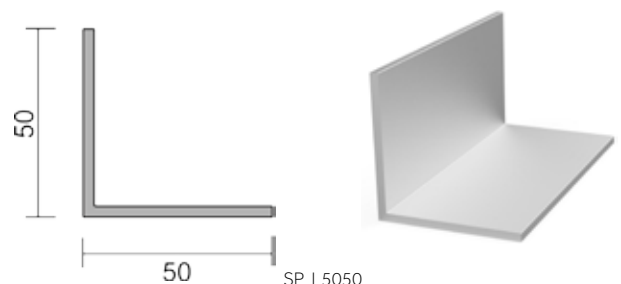
SP L5050 L-profile 50 x 50 x 2 mm
