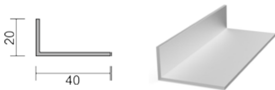
SP L4020 L-profile 40 x 20 x 2 mm
